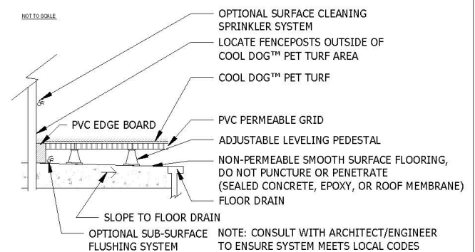
ELEVATED PLATFORM INSTALLATION
